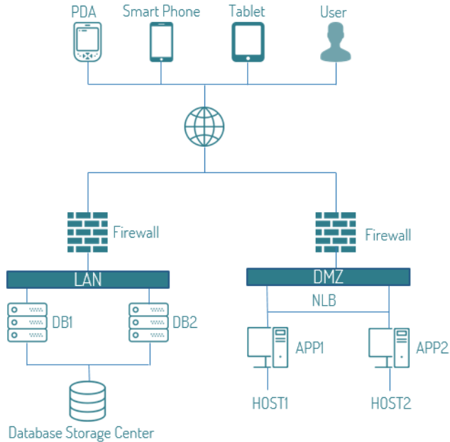
High Available Architecture
